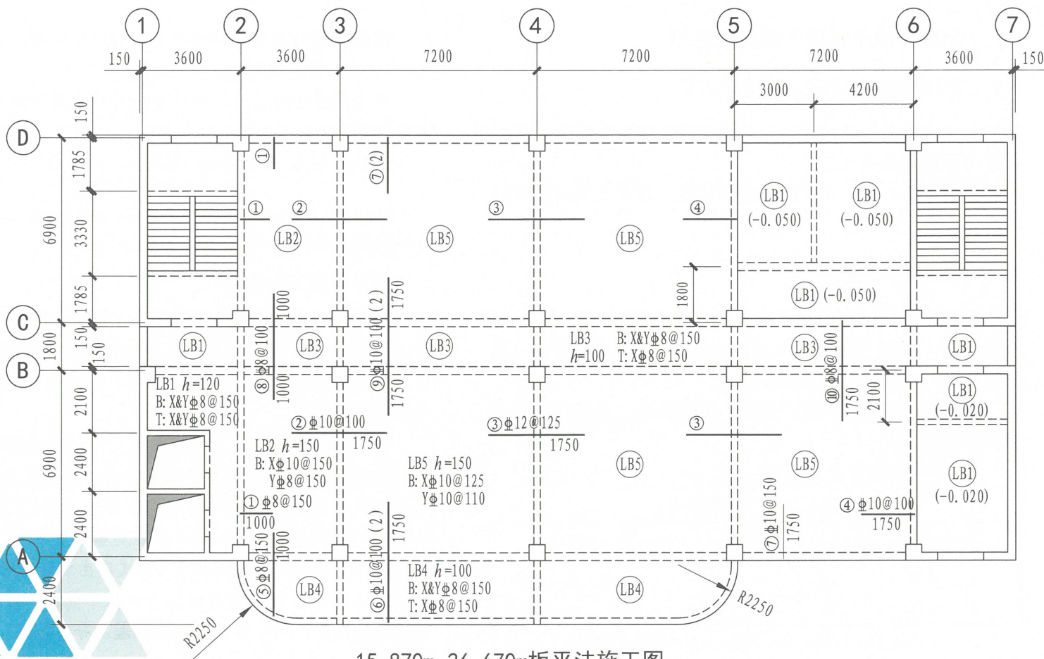
15.870m~26.670m板平法施工图
