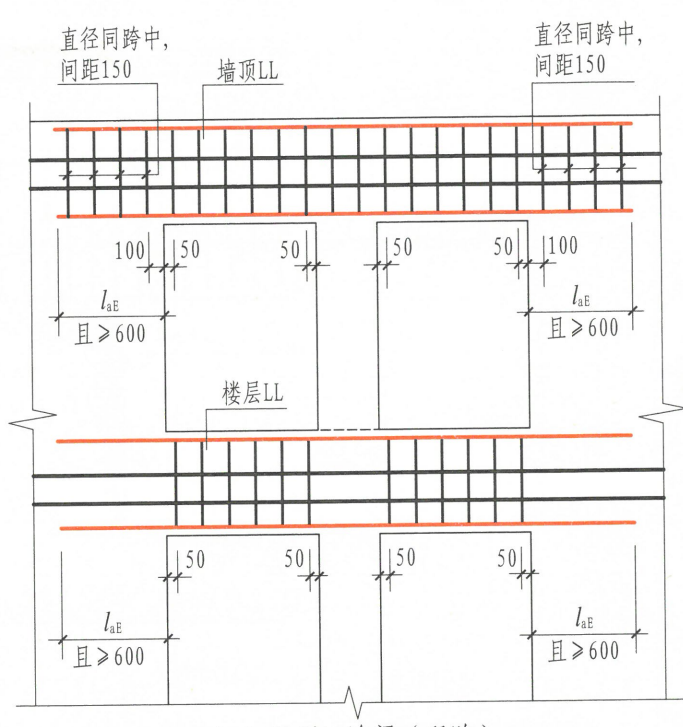
(c) 双洞口连梁 (双跨)
